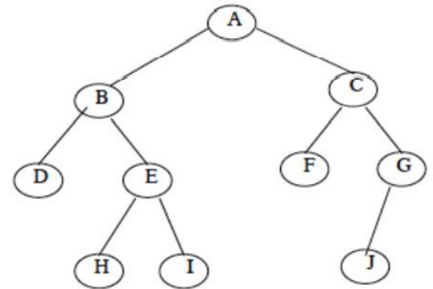
Fig 2: Binary Tree
