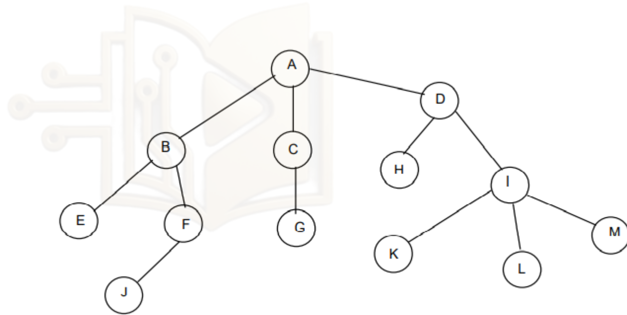
Fig. Tree
