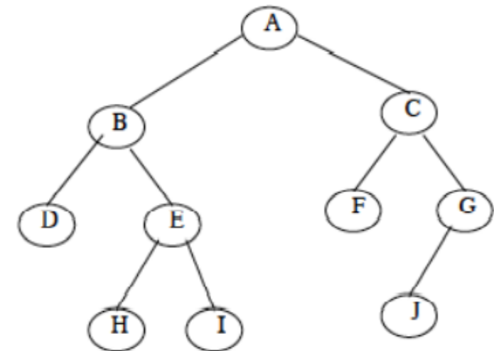
Fig10: Binary Tree
