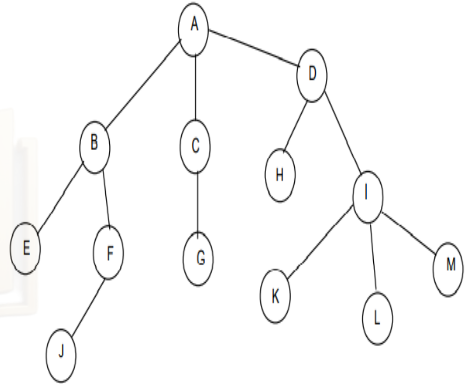
Fig. Tree
