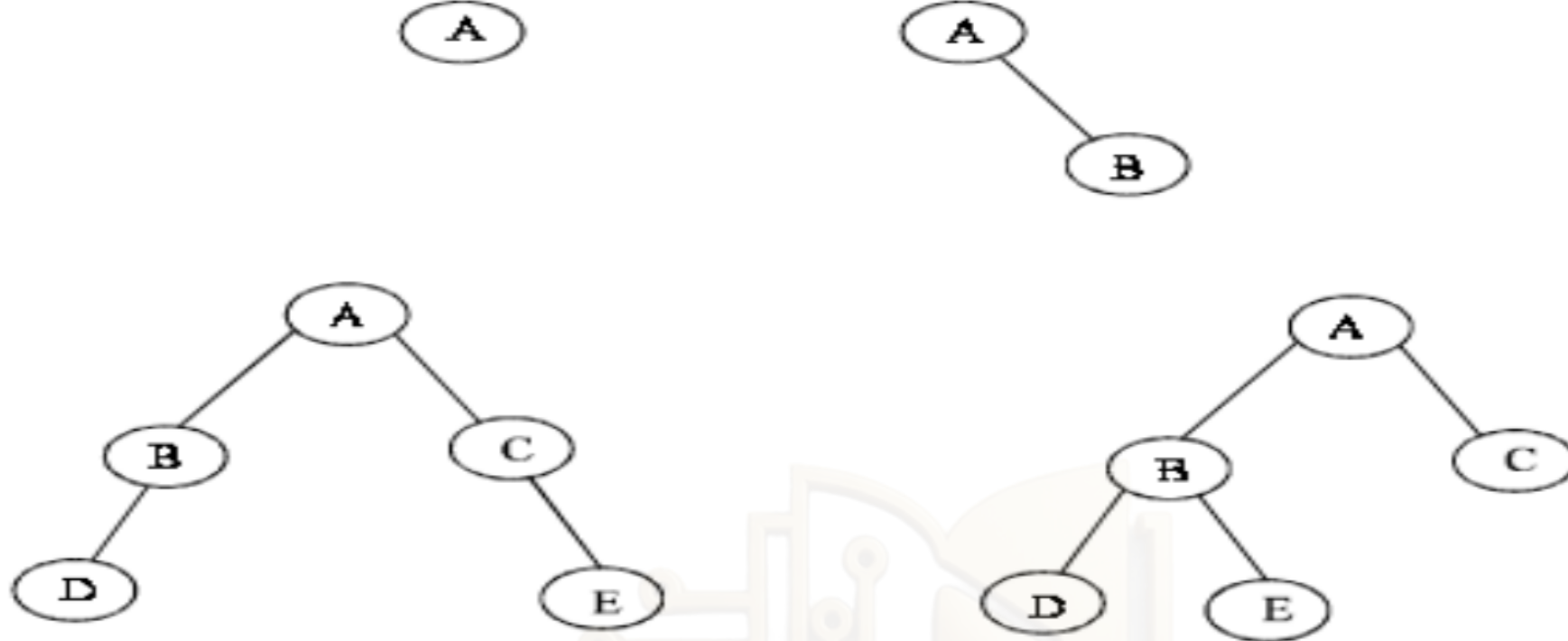
Fig17: AVL Trees
