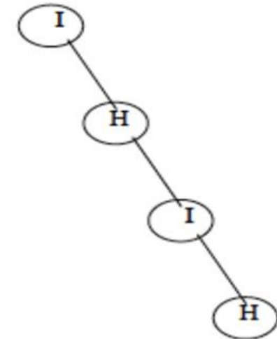
Fig7: Right Skewed
