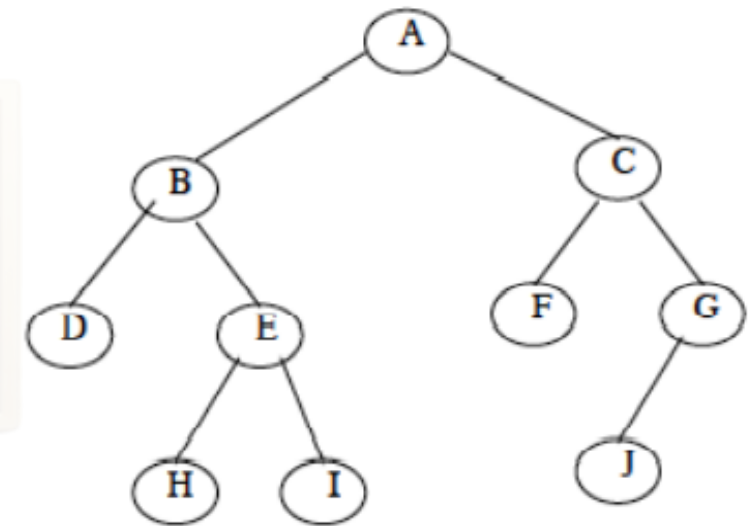
Fig10: Binary Tree
